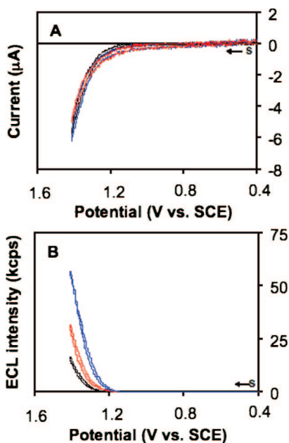
Figure 1. Cyclic voltammograms (frame A) and ECL intensity (kilocounts per second, kcps) vs potential curves (frame B) at an ITO electrode in a solution before (black curves) and after injecting 1 nM (red curves) and 2 nM (blue curves) Pt NPs. The solution contains 0.1 M NaClO 4 , phosphate buffer (pH 7.0), 10 μM Ru(bpy) 3 (ClO 4 ) 2 , and 50 mM TPrA. Potential scan rate = 20 mV/s from point s.
